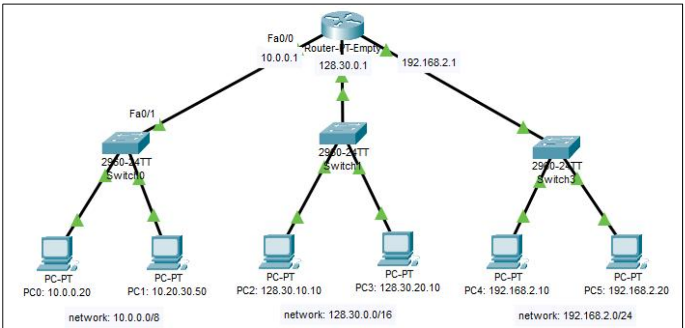
Fig: Topology of Class A, B and C Network
